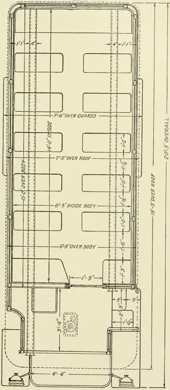
Fig. 18. Diagram Showing Interior Arrangement of Leeds Trackless Trolley Cars
